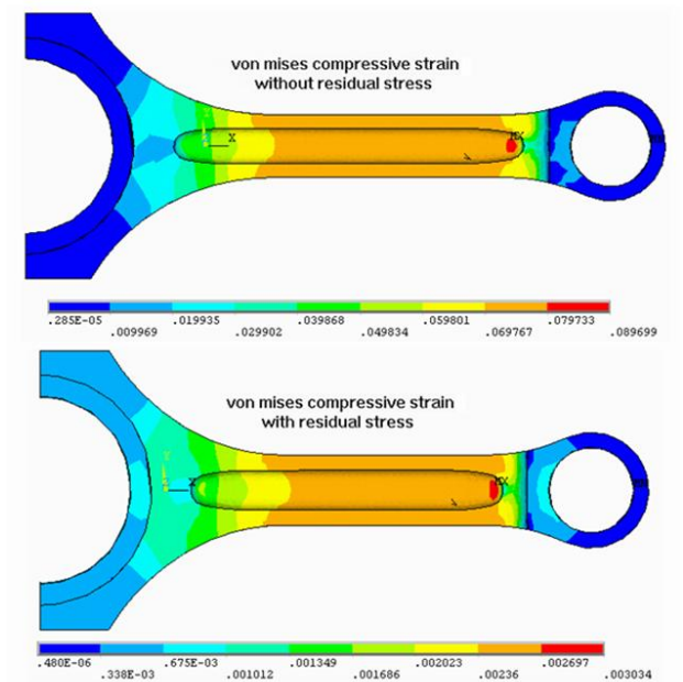
Fig11. Von mises strain distribution, before and after application of residual compressive stress.
