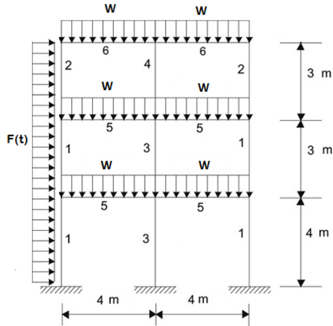
Figure 15. Topology of the six story frame
