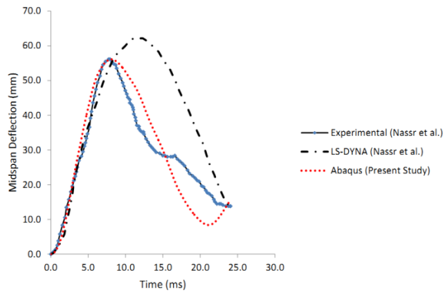
Figure 8. Mid-span deflection of C1 column
