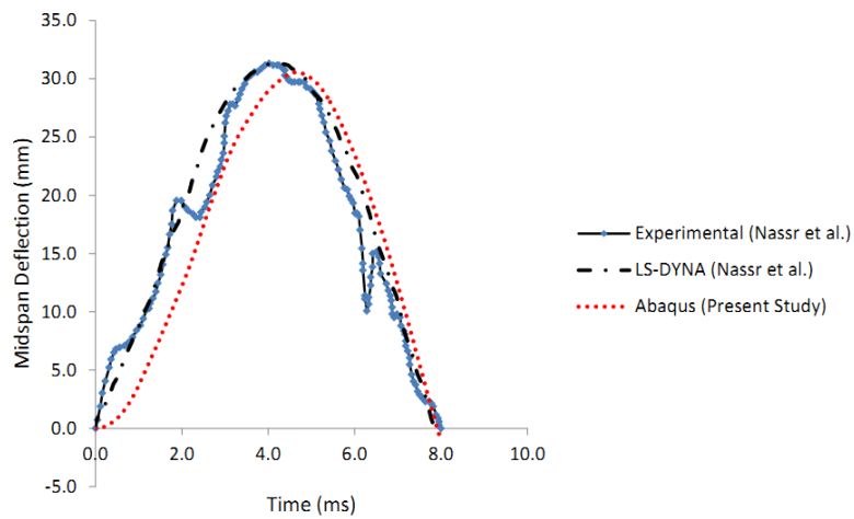
Figure 9. Mid-span deflection of C2 column
